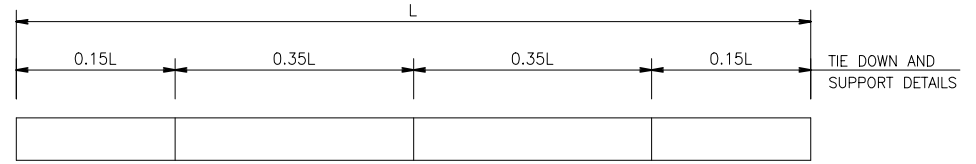
3-POINT SUPPORT
