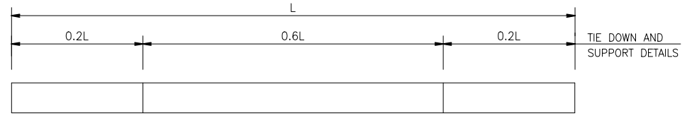
2-POINT SUPPORT
