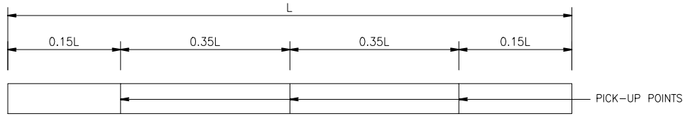
3-POINT PICK-UP
